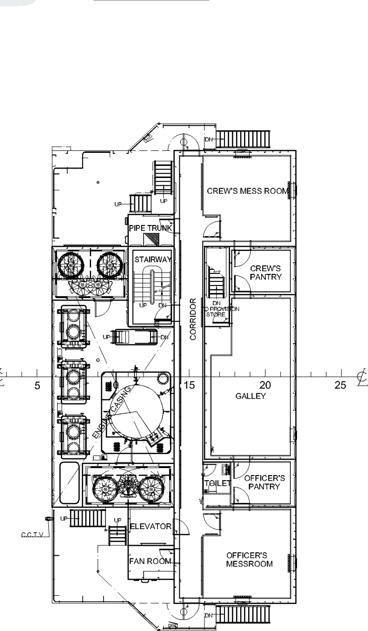
B - DECK
