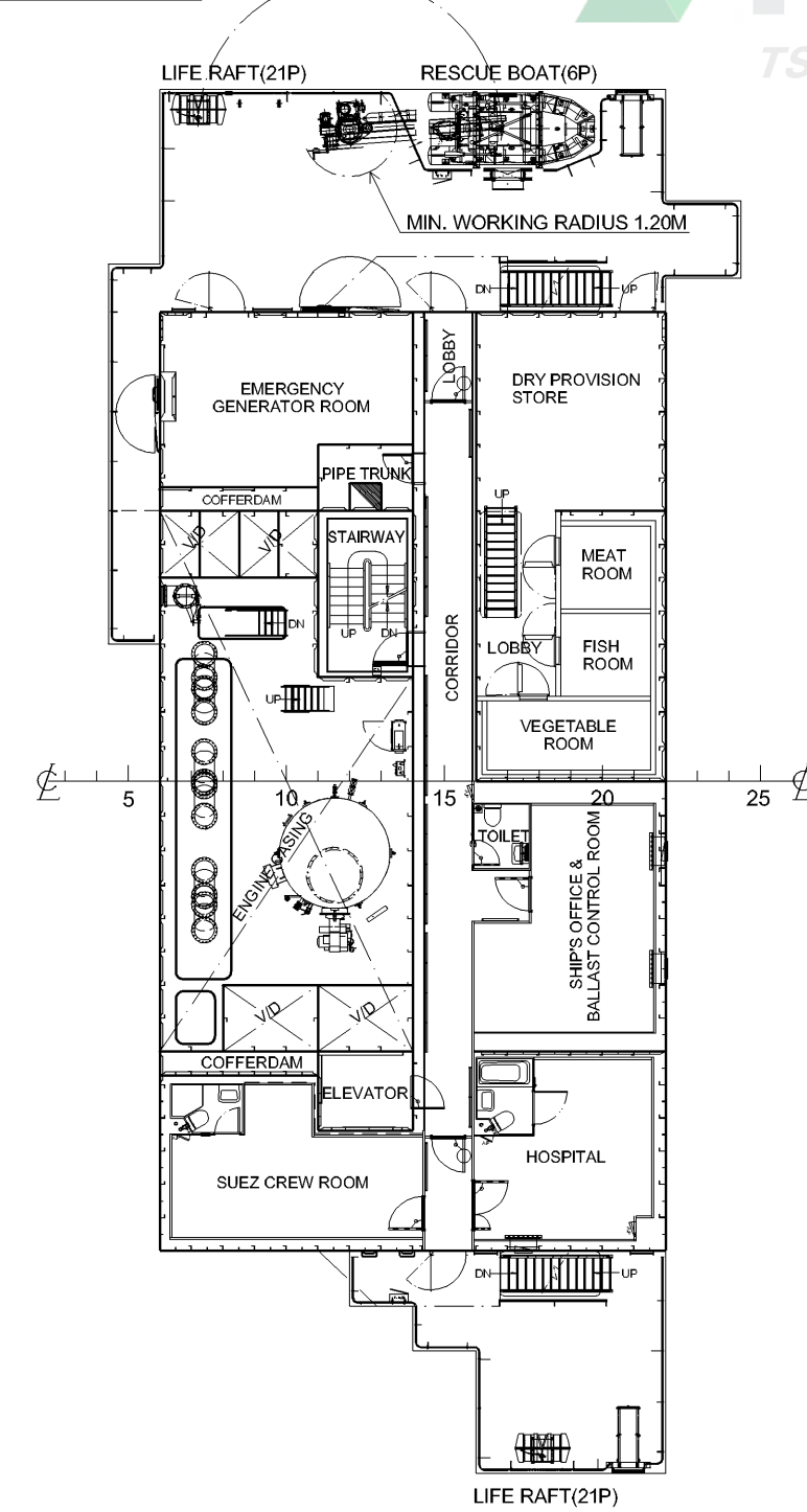
A - DECK
