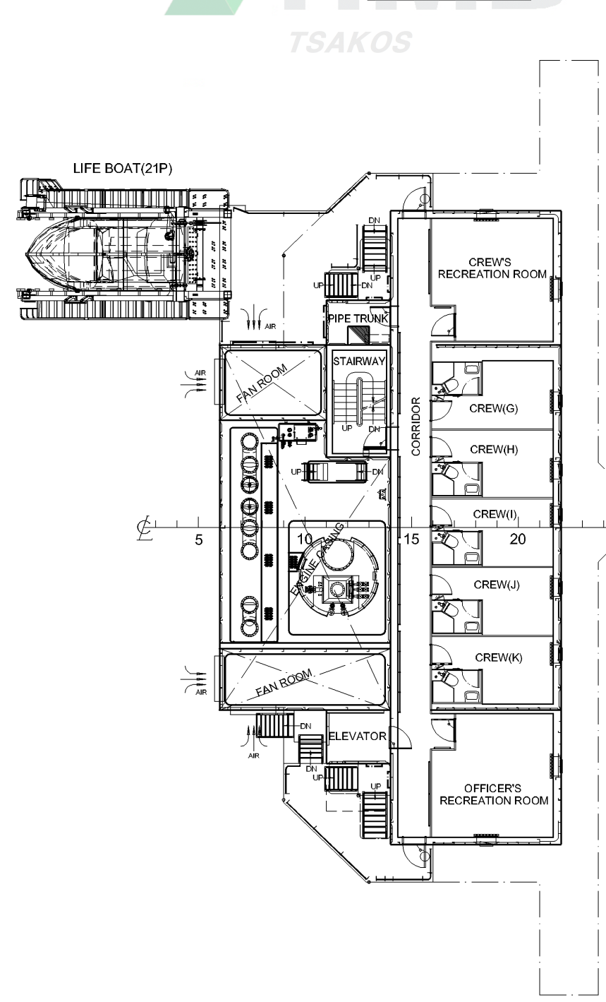
C - DECK
