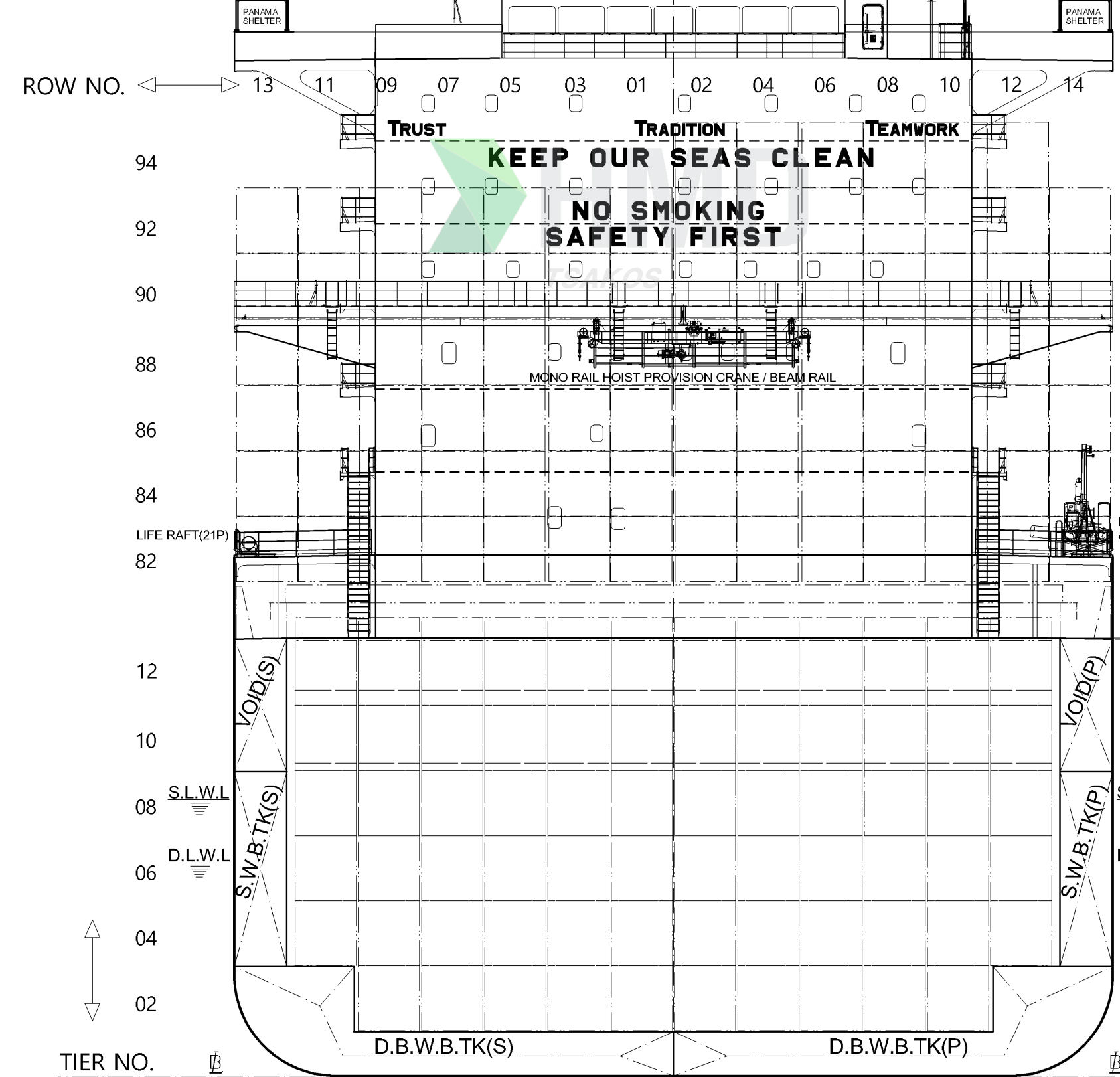
MIDSHIP SECTION
