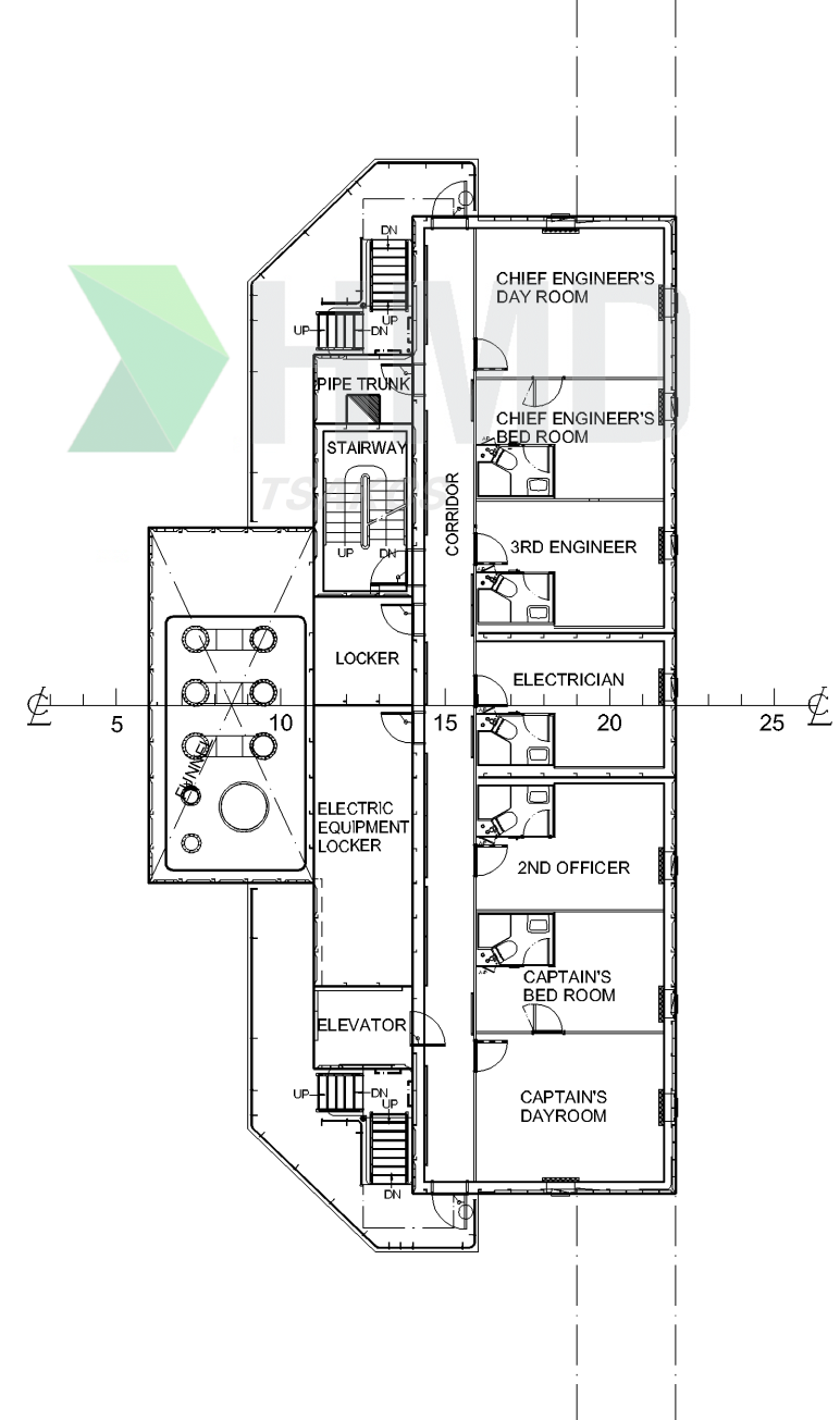
F - DECK
