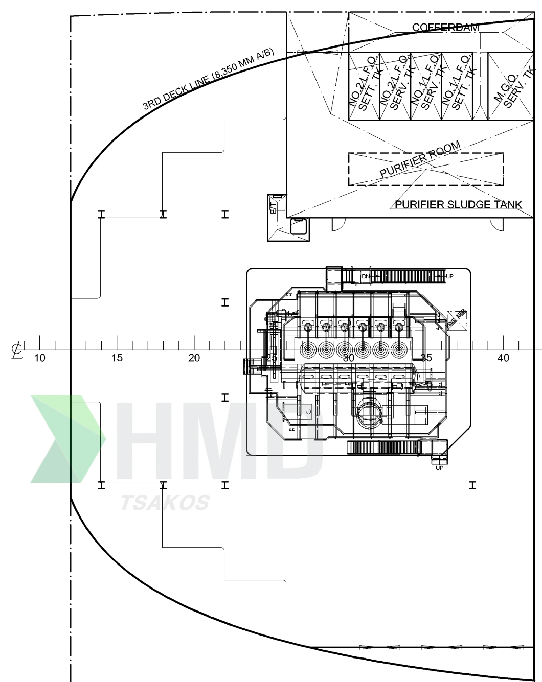
E/R 3RD DECK (8,350MM A/B)
