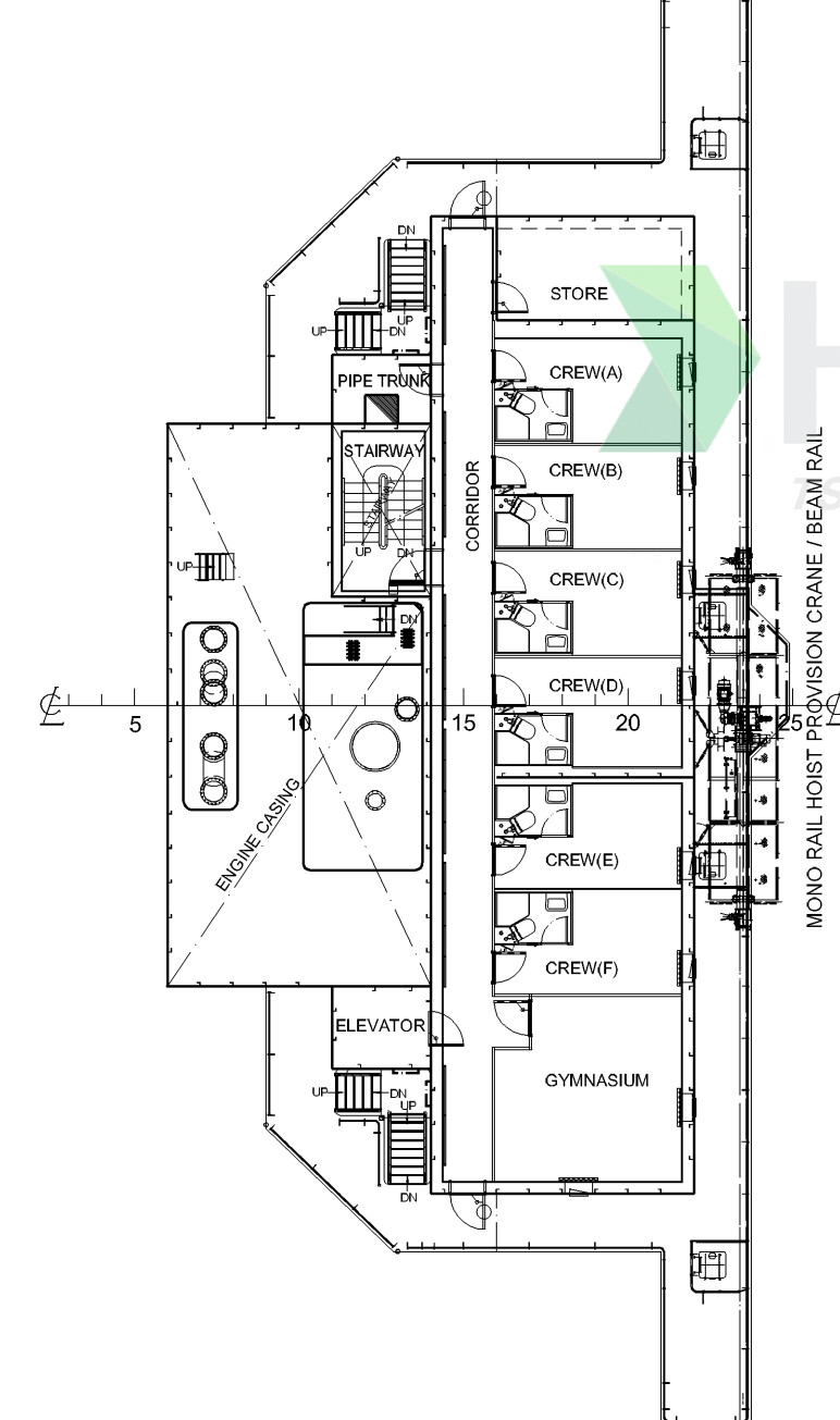
D - DECK
