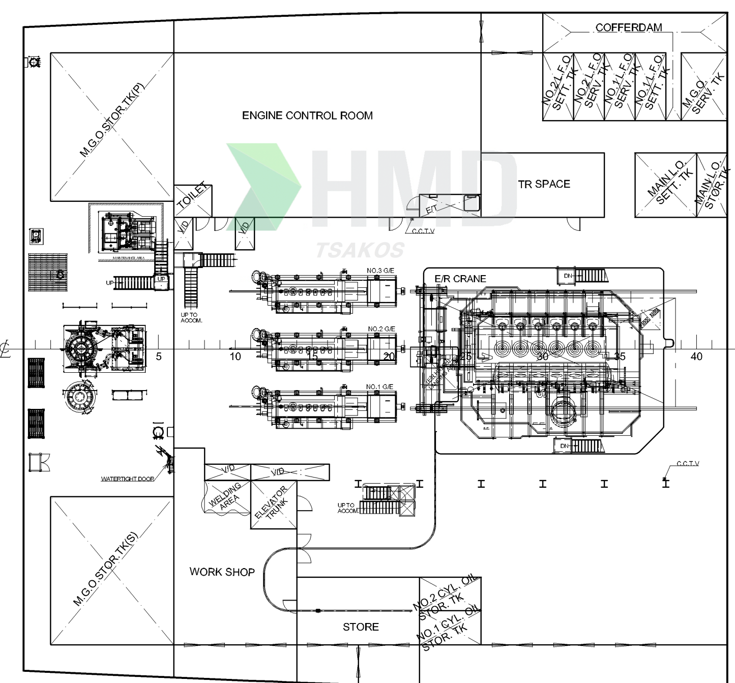
E/R 2ND DECK (12,127MM A/B)
